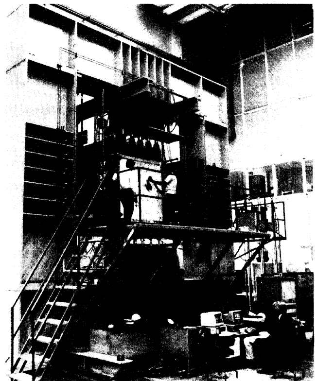
Fig. 21 — The shell element tester
