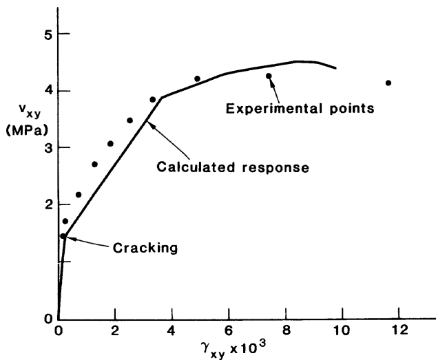
Fig. 15 — Comparison of calculated and observed response of Specimen PV20 (1 MPa = 145 psi)
