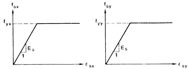
Fig. 6 — Stress-strain relationships for reinforcement
