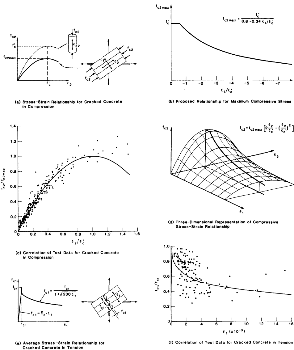
Fig. 11 — Stress-strain relationships for cracked concrete
