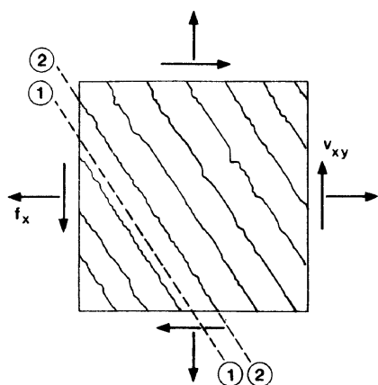
(a) Stresses Applied to Cracked Element
