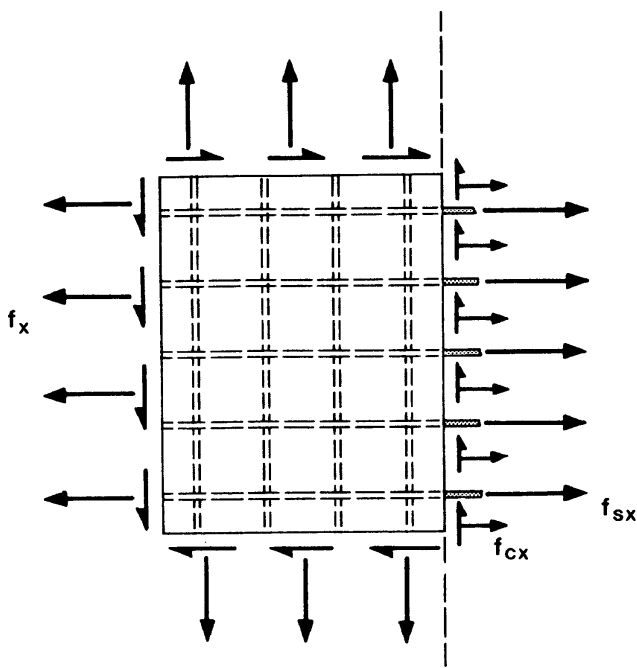
Fig. 4 — Free-body diagram of part of element
