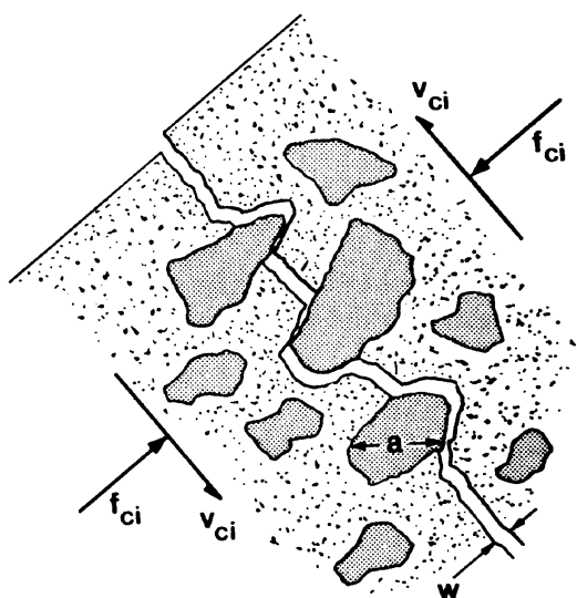
Fig. 13 — Transmitting shear stresses across crack by aggregate interlock
