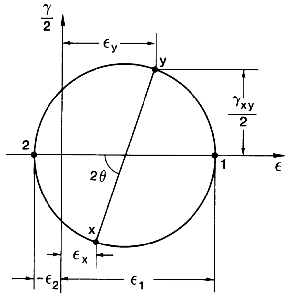
(b) Mohr's Circle for Average Strains
