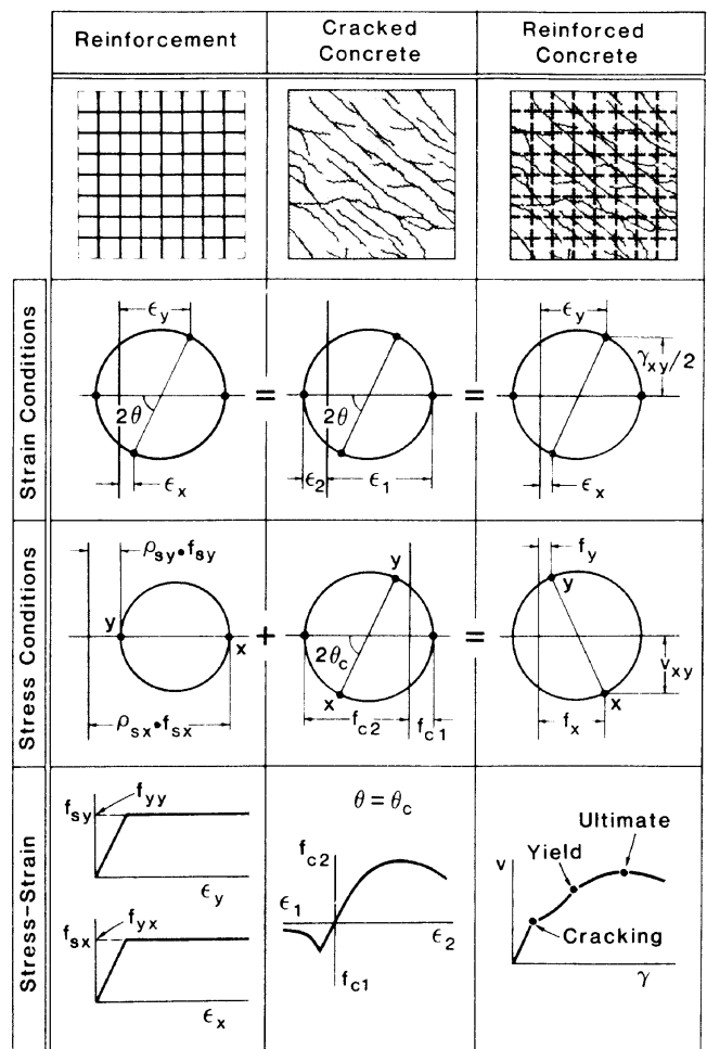
Fig. 20 — The modified compression-field theory for membrane elements
