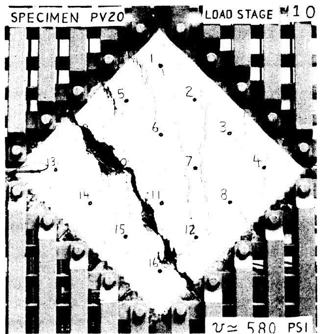
Fig. 16 — Specimen PV20 after failure
