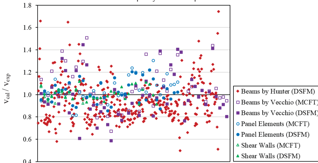
Figure 8 — Calculated-to-measured load capacity for MCFT and DSFM
