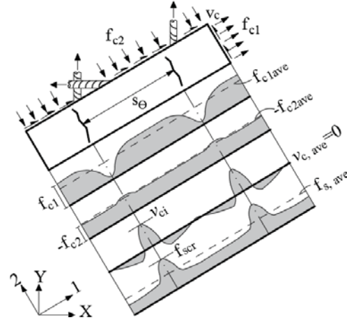
Figure 6 — Stress conditions at crack locations and between cracks
